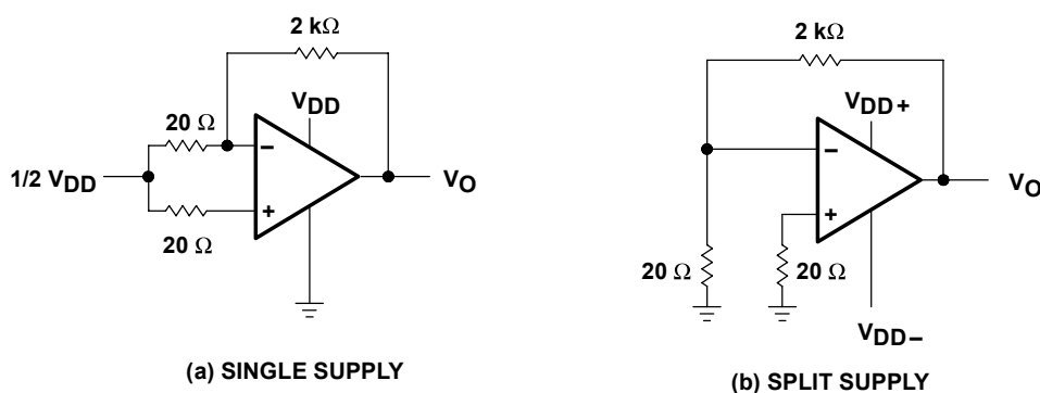
Figure 2. Noise-Test Circuit
