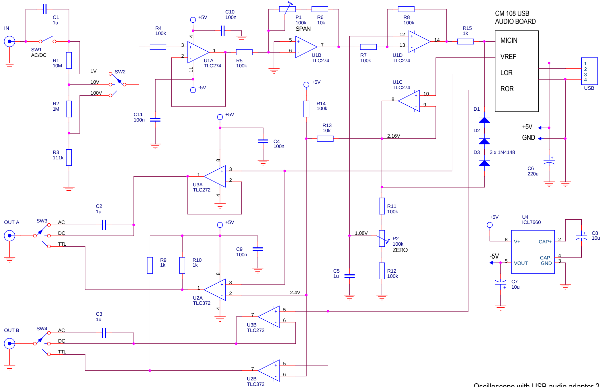
Oscilloscope with USB audio adapter 2
