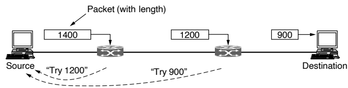
Figure 5-42. Path MTU discovery.
