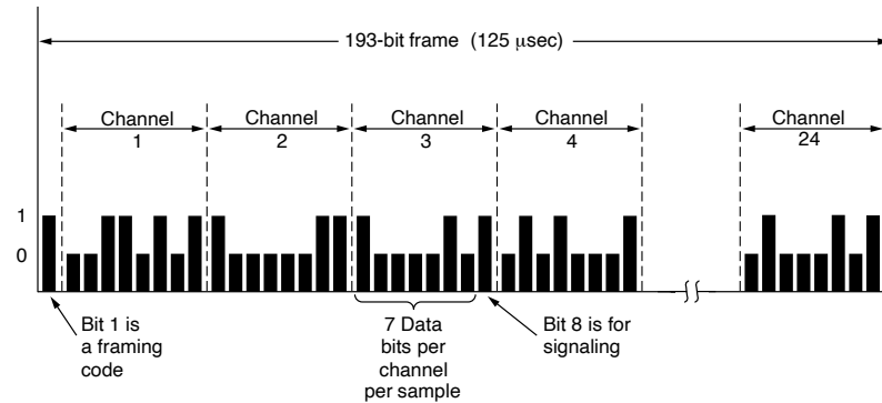
Figure 2-32. The T1 carrier (1.544 Mbps).
