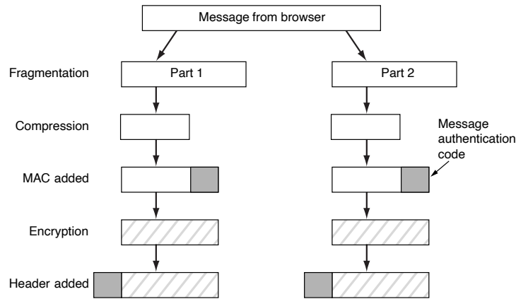
Figure 8-50. Data transmission using SSL.
