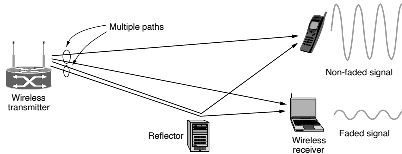
Figure 1-23. Multipath fading.
