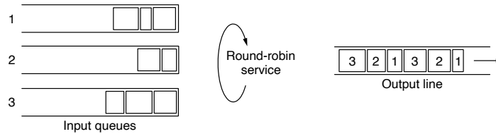
Figure 5-28. Round-robin fair queueing.
