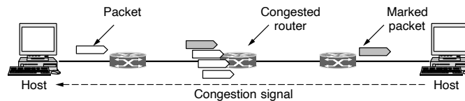
Figure 5-25. Explicit congestion notification
