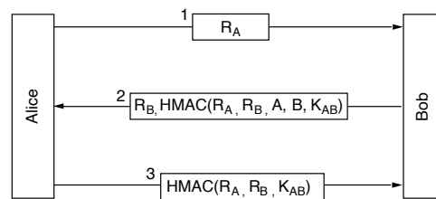
Figure 8-33. Authentication using HMACs.
