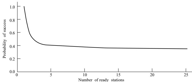
Figure 4-9. Acquisition probability for a symmetric contention channel.
