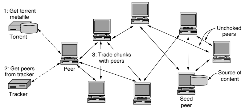
Figure 7-47. BitTorrent.
