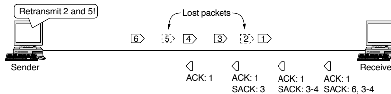
Figure 6-48. Selective acknowledgements.
