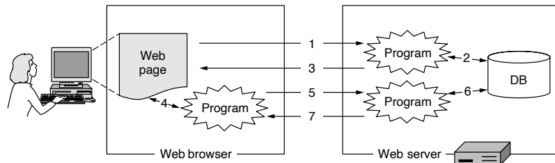
Figure 7-23. Dynamic pages.
