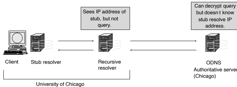
Figure 7-8. Oblivious DNS.
