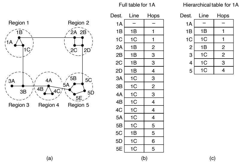
Figure 5-14. Hierarchical routing.
