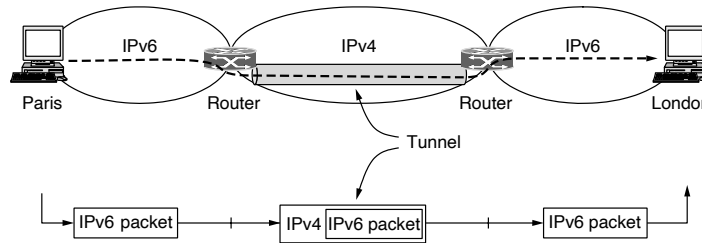
Figure 5-38. Tunneling a packet from Paris to London.
