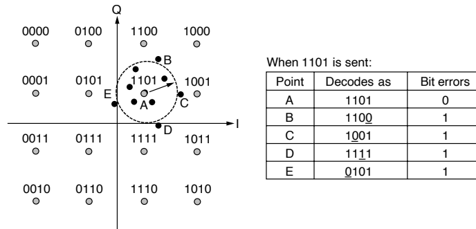
Figure 2-18. Gray-coded QAM-16.
