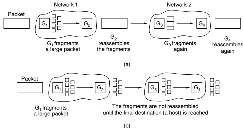
Figure 5-40. (a) Transparent fragmentation. (b) Nontransparent fragmentation.
