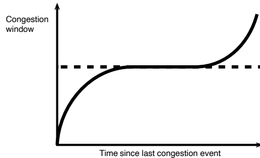
Figure 6-49. Evolution of TCP CUBIC Congestion Window.
