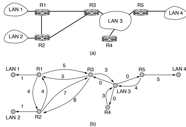
Figure 5-65. (a) An autonomous system. (b) A graph representation of (a).
