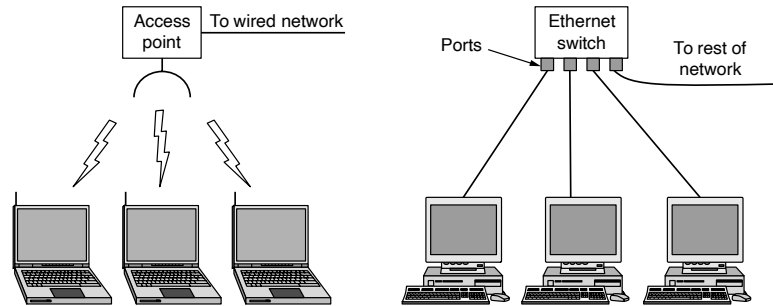
Figure 1-7. Wireless and wired LANs. (a) 802.11. (b) Switched Ethernet.
