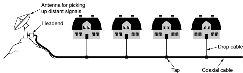
Figure 2-44. An early cable television system.
