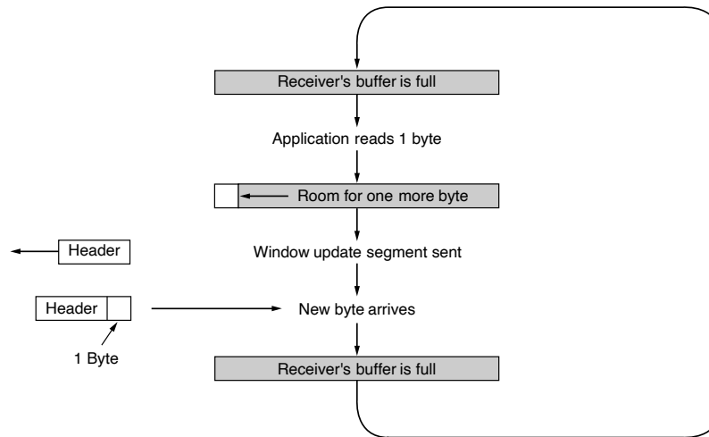
Figure 6-41. Silly window syndrome.
