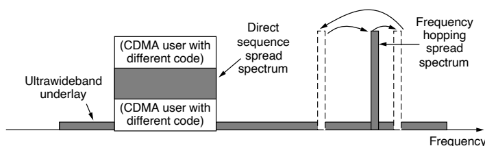
Figure 2-9. Spread spectrum and ultra-wideband (UWB) communication.
