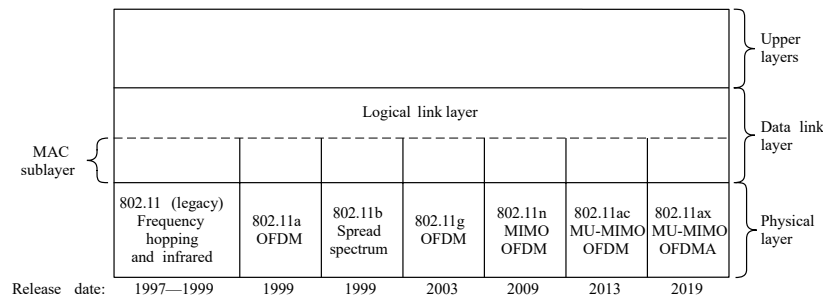
Figure 4-24. Part of the 802.11 protocol stack.
