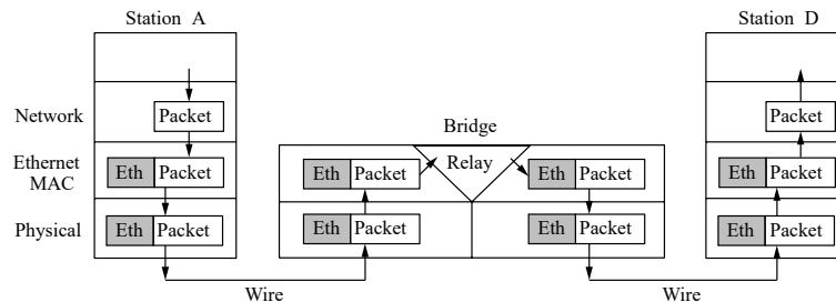
Figure 4-34. Protocol processing at a bridge.
