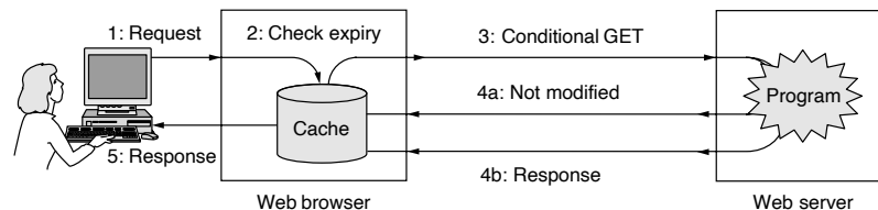
Figure 7-28. HTTP caching.
