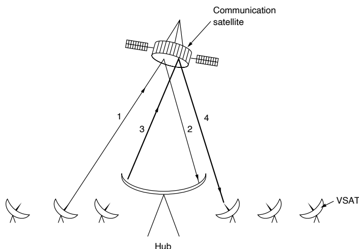
Figure 2-50. VSATs using a hub.
