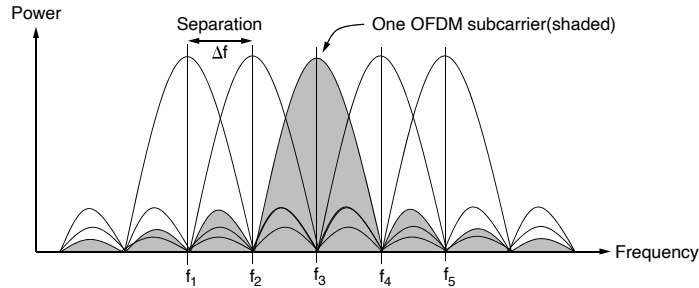
Figure 2-20. Orthogonal frequency division multiplexing (OFDM).
