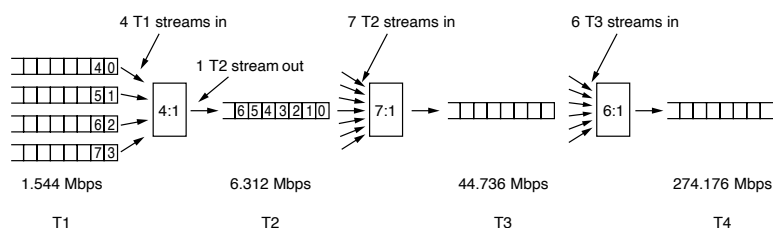
Figure 2-33. Multiplexing T1 streams into higher carriers.
