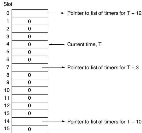
Figure 6-54. A timing wheel.
