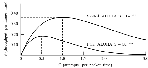
Figure 4-3. Throughput versus offered traffic for ALOHA systems.
