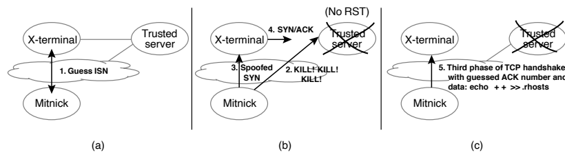
Figure 8-6. Mitnick's attack
