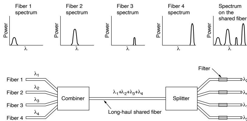
Figure 2-23. Wavelength division multiplexing.
