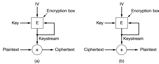
Figure 8-18. A stream cipher. (a) Encryption. (b) Decryption.
