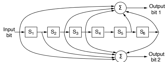
Figure 3-7. The NASA binary convolutional code used in 802.11.
