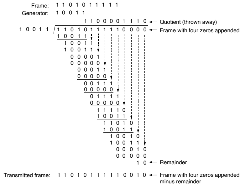
Figure 3-9. Example calculation of the CRC.
