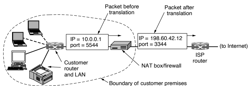
Figure 5-56. Placement and operation of a NAT box.
