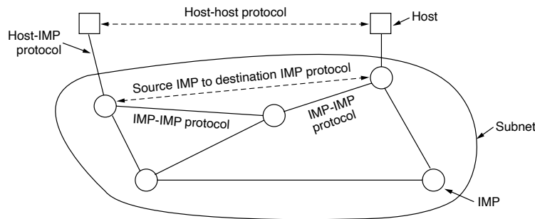
Figure 1-13. The original ARPANET design.
