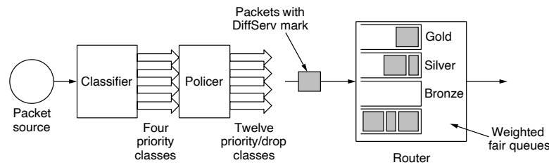
Figure 5-35. A possible implementation of assured forwarding.
