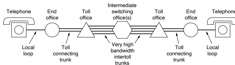
Figure 2-25. A typical circuit route for a long-distance call.
