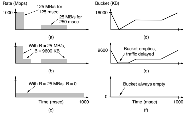
Figure 5-24. (a) Traffic from a host. Output shaped by a token bucket of rate 200 Mbps and capacity (b) 9600 KB and (c) 0 KB. Token bucket level for shaping with rate 200 Mbps and capacity (d) 16,000 KB, (e) 9600 KB, and (f) 0 KB.
