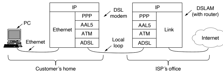
Figure 3-26. ADSL protocol stacks.
