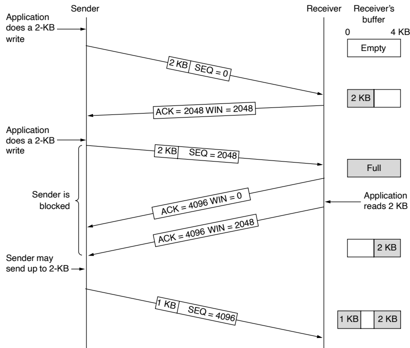
Figure 6-40. Window management in TCP.
