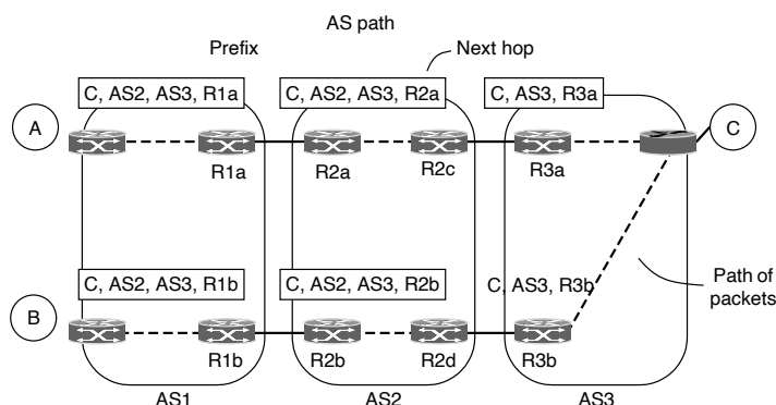
Figure 5-69. Propagation of BGP route advertisements.
