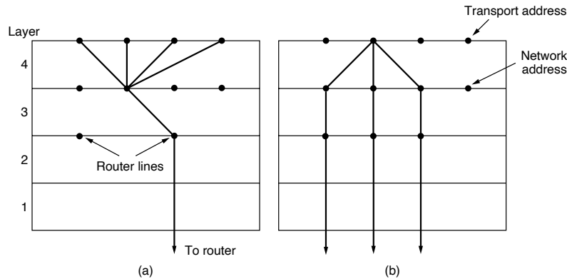
Figure 6-17. (a) Multiplexing. (b) Inverse multiplexing.
