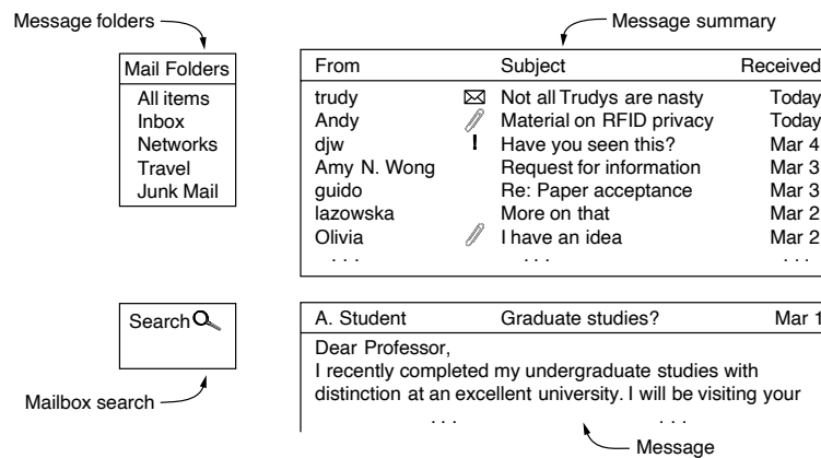
Figure 7-11. Typical elements of the user agent interface.
