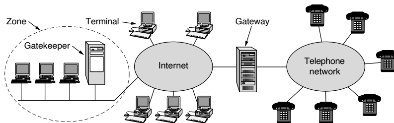
Figure 7-36. The H.323 architectural model for Internet telephony.
