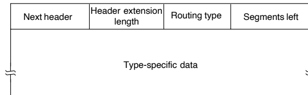
Figure 5-60. The extension header for routing.
