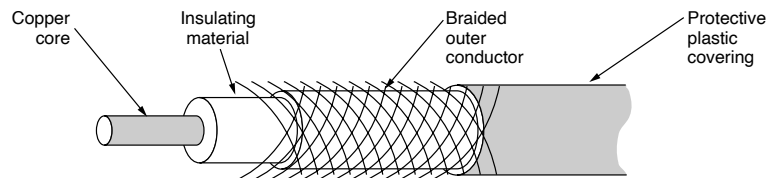
Figure 2-2. A coaxial cable.
