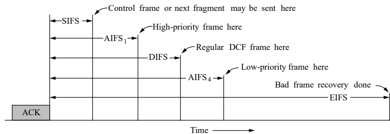
Figure 4-28. Interframe spacing in 802.11.
