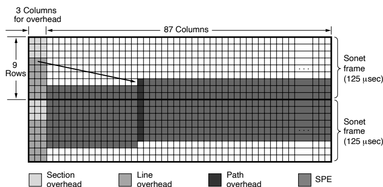
Figure 2-34. Two back-to-back SONET frames.
