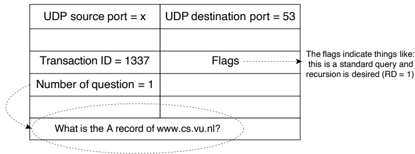
Figure 8-3. A DNS request for www.cs.vu.nl .
