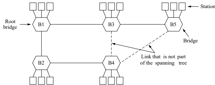
Figure 4-36. A spanning tree connecting five bridges. The dashed lines are links that are not part of the spanning tree.
