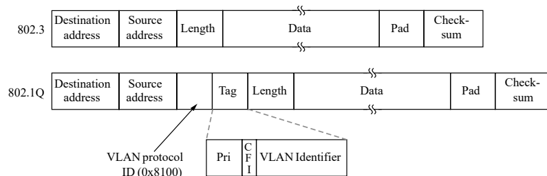
Figure 4-41. The 802.3 (legacy) and 802.1Q Ethernet frame formats.
