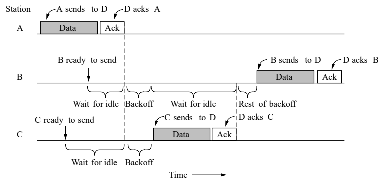
Figure 4-25. Sending a frame with CSMA/CA.
