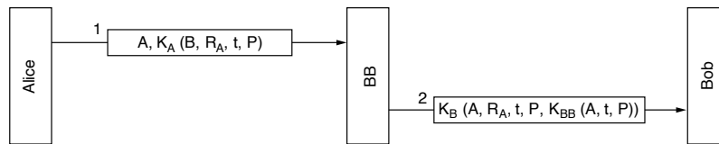
Figure 8-21. Digital signatures with Big Brother.
