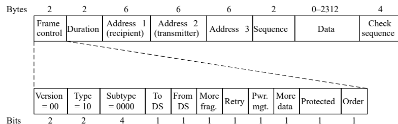
Figure 4-29. Format of the 802.11 data frame.
