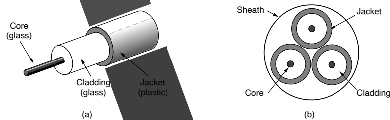
Figure 2-6. (a) Side view of a single fiber. (b) End view of a sheath with three fibers.
