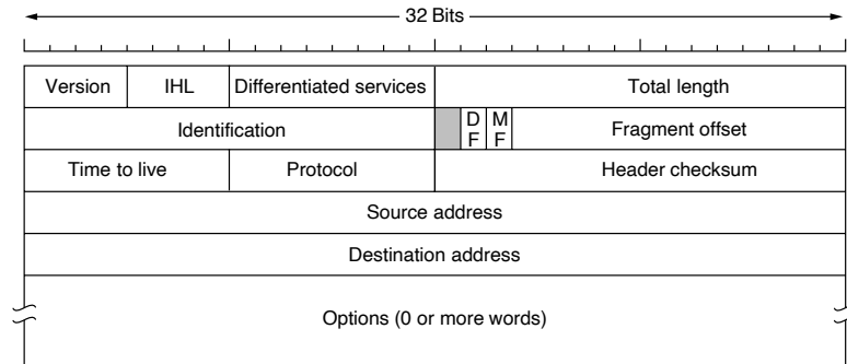
Figure 5-47. The IPv4 (Internet Protocol version 4) header.
